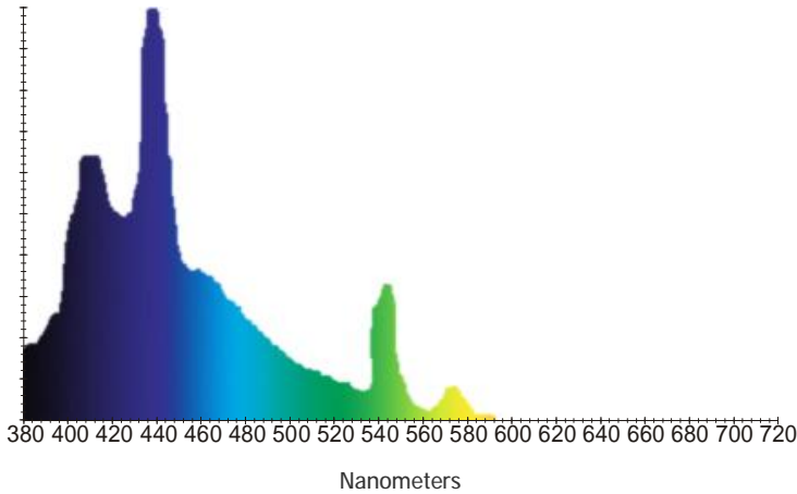
Spectral Energy Distribution
