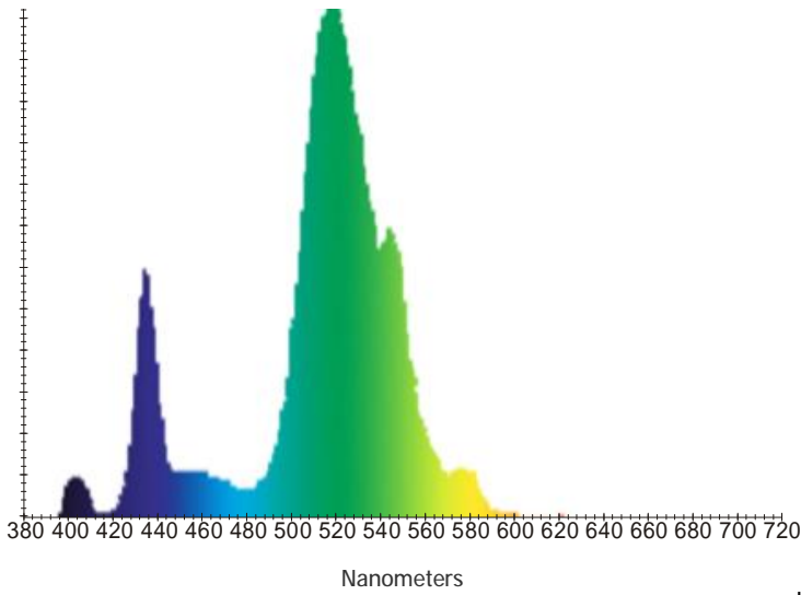
Discharge With Low Pressure Mercury Vapor
