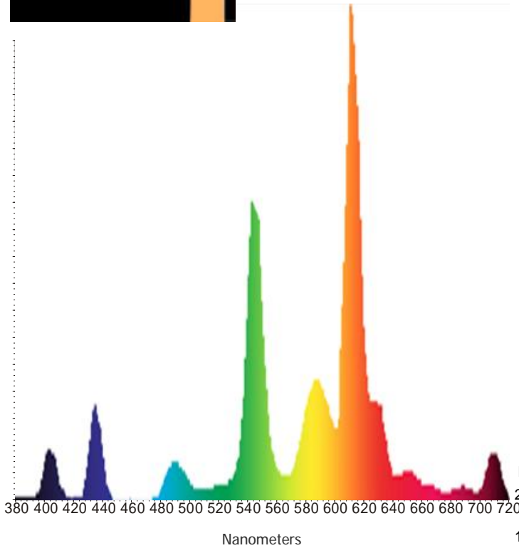
Spectral Energy Distribution
