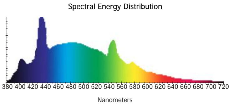
Discharge With Low Pressure Mercury Vapor
