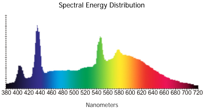
Discharge With Low Pressure Mercury Vapor
