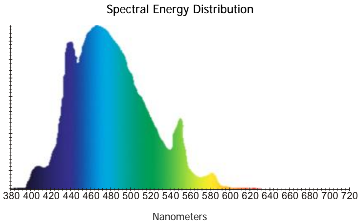
Discharge With Low Pressure Mercury Vapor
