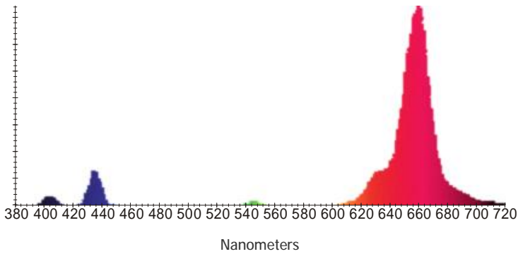
Discharge With Low Pressure Mercury Vapor
