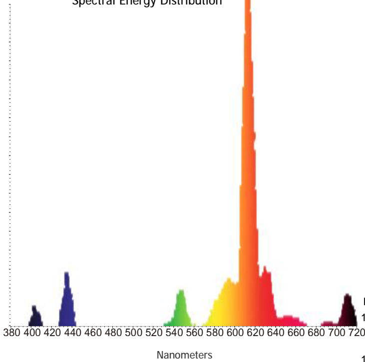
Discharge With Low Pressure Mercury Vapor
