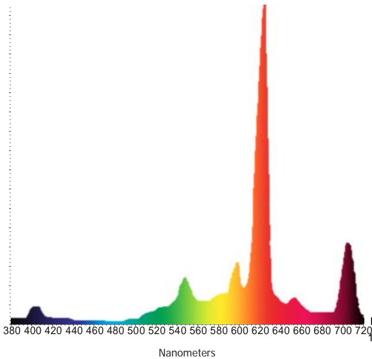
Discharge With Low Pressure Mercury Vapor
