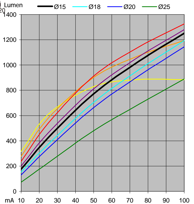
Luminous Flux 1 m - diam. 15 mm
